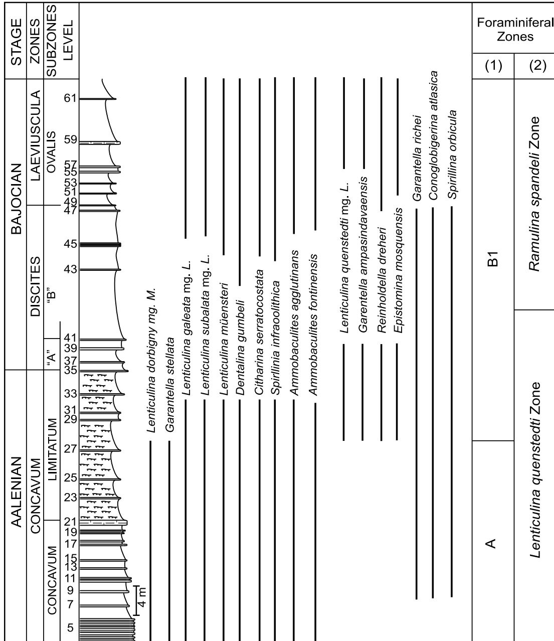
Fig. 9. Distribution of foraminifers across the Aalenian/Bajocian boundary in the Central High Atlas (modified after Amhoud, Boutakiout, 1994) and foraminiferal zones established for: (1) Central High Atlas (Amhoud, Boutakiout, 1994); (2) Lusitanian Basin (Canales, Henriques, 2013)
