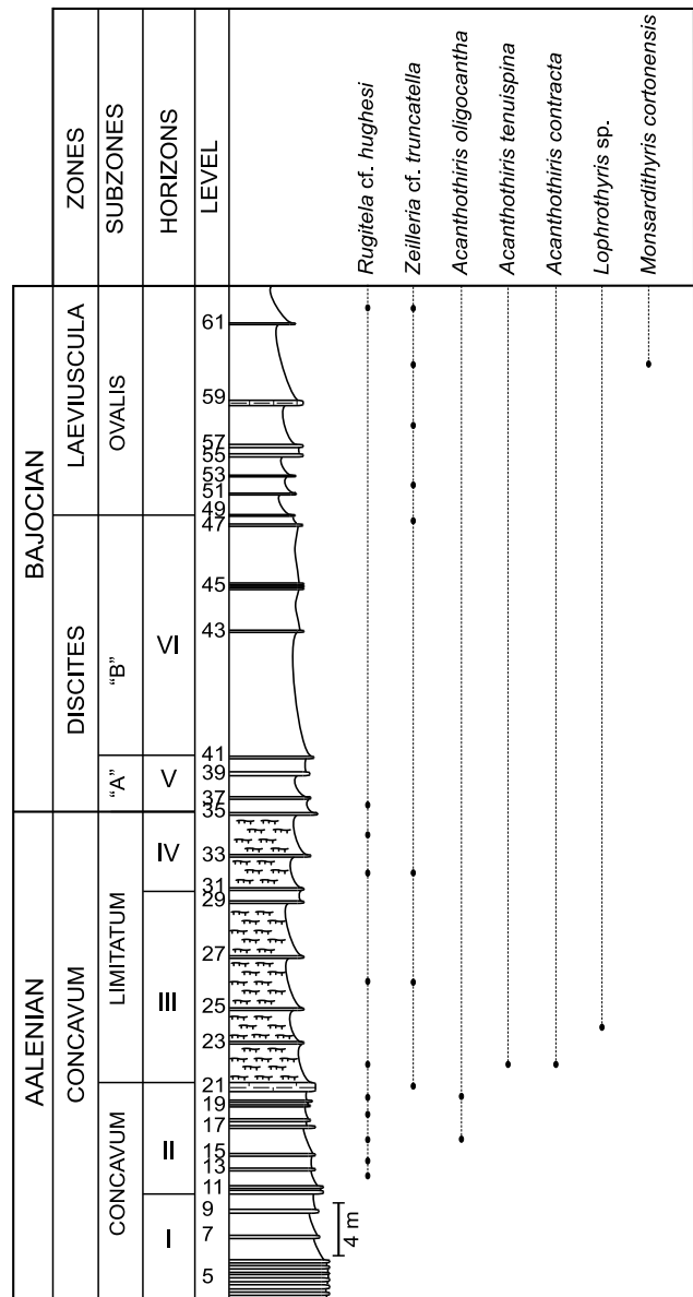
Fig. 4. Distribution of brachiopods across the Aalenian/Bajocian boundary in the Central High Atlas (Sadki, Almeras, 1992)
